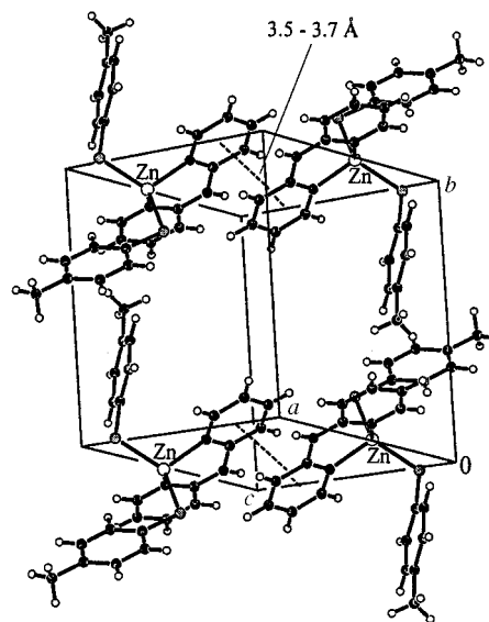
Fig. 7 The crystal packing diagram of [\text{Zn}(\text{dpa})(4\text{-MeC}_6\text{H}_4\text{S})_2] 1d shows a self-assembled infinite 1-D tape structure generated by extensive aromatic \pi\text{–}\pi interactions.
